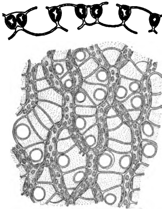
FIG. 345. — Leaf of Sphagnum ; \times 600 .
